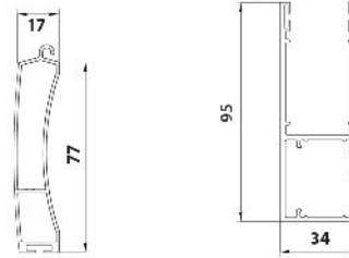
SLAT (INSULATED)
