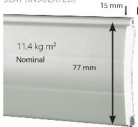
SLAT (INSULATED)
