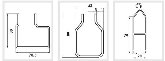
SLAT (INSULATED)
