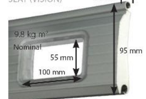
SLAT (VISION)
